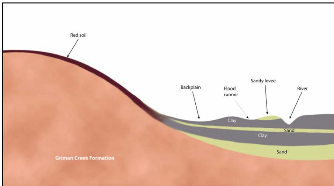
Figure 3. Conceptual cross section of the western Macintyre alluvia (Andrew Biggs, NRW, personal communication).
