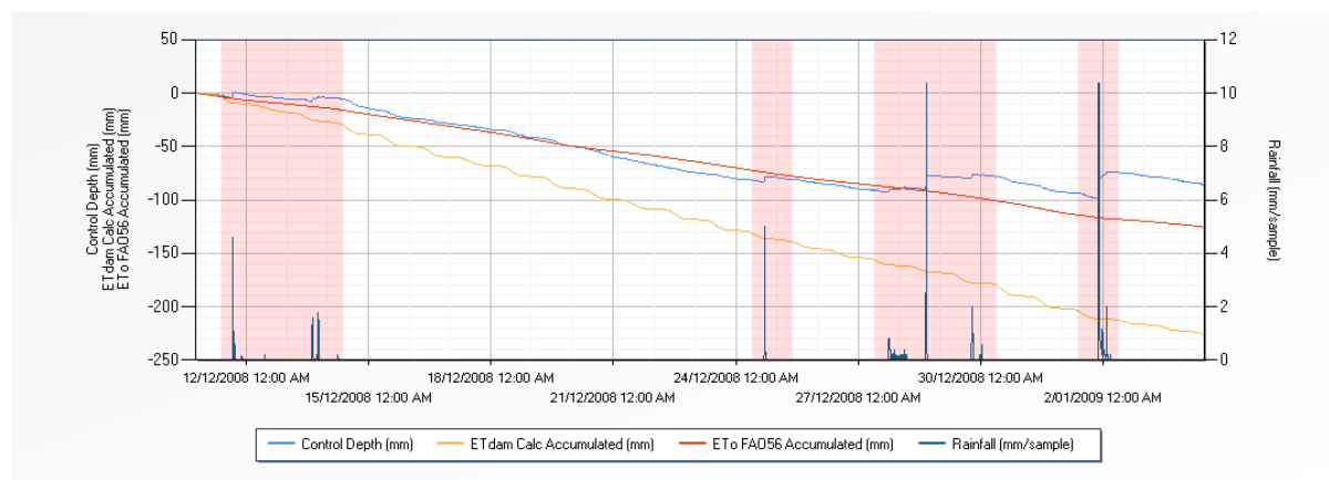
Figure 3 – Example of the Evapcalc software being used to determine seepage and evaporation.
